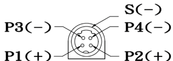
Output cable plug pin assignment
